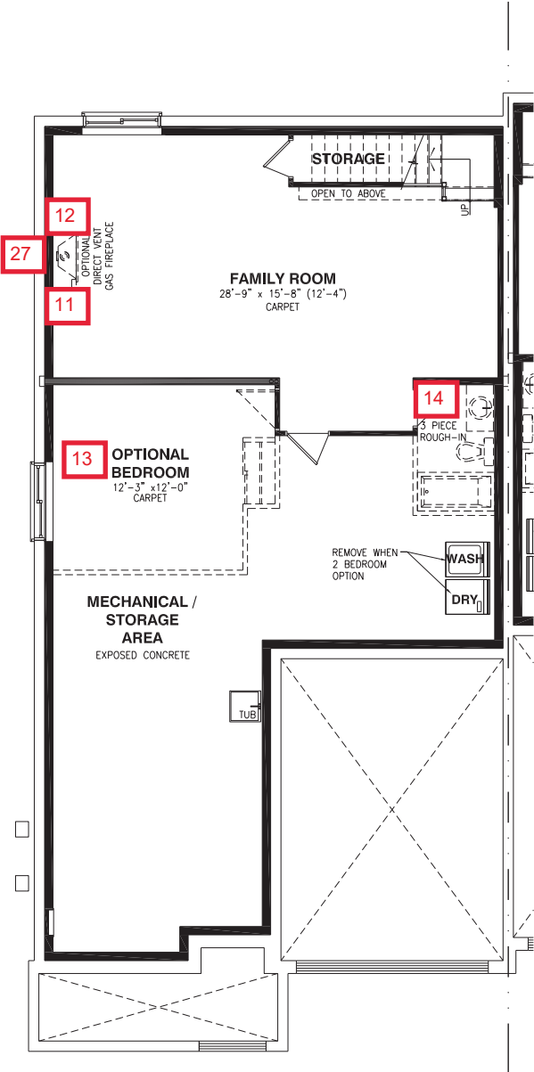
BASEMENT FLOOR
