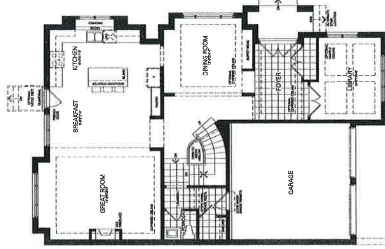
GROUND FLOOR A
