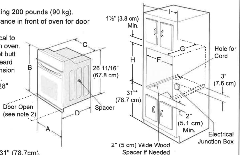
Figure 1 30" Single Wall Ovens (Double ovens see Figure 2)
