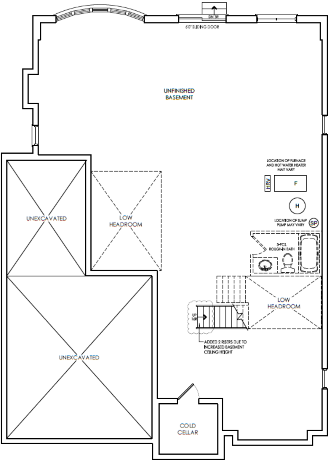
BASEMENT FLOOR ELEV. 'A' W/ WALK-OUT BASEMENT (LOT 20N)
