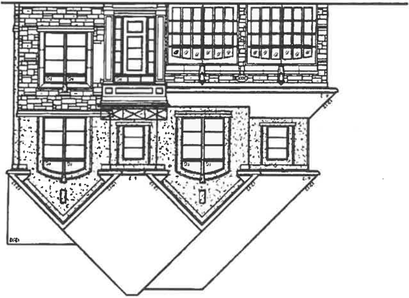
UPGRADED FRONT ELEVATION 'C' FOR LOT 90W
