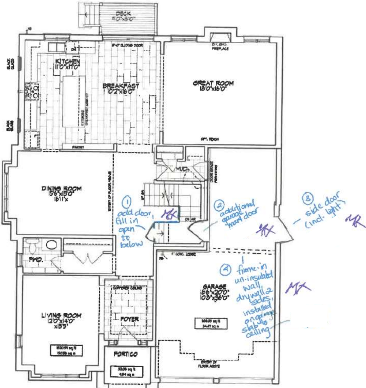
GROUND FLOOR PLAN, EL. 'A'
