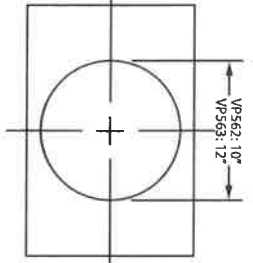
VP562/VP563 transition centers outlet over top of hood
