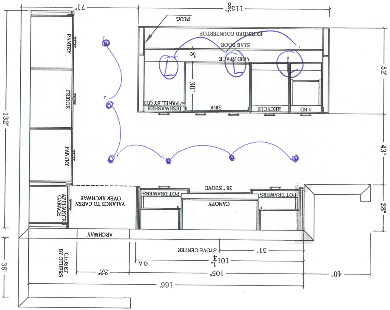
KITCHEN PLAN
