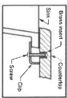
Detail of Mounting Clip
