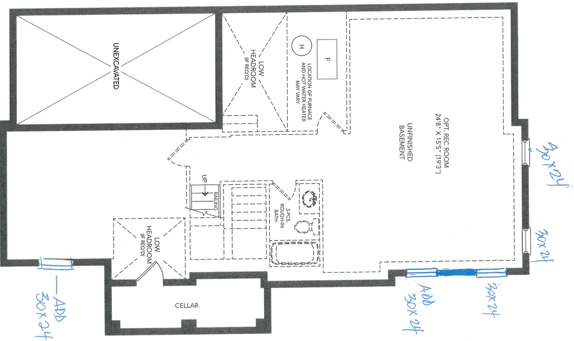
BASEMENT PLAN ELEV. 'A'
