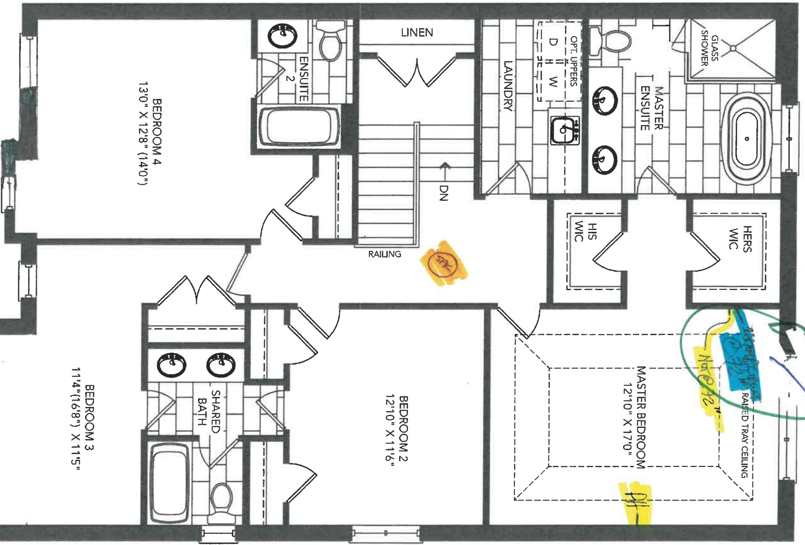
SECOND FLOOR PLAN ELEV. A/B
