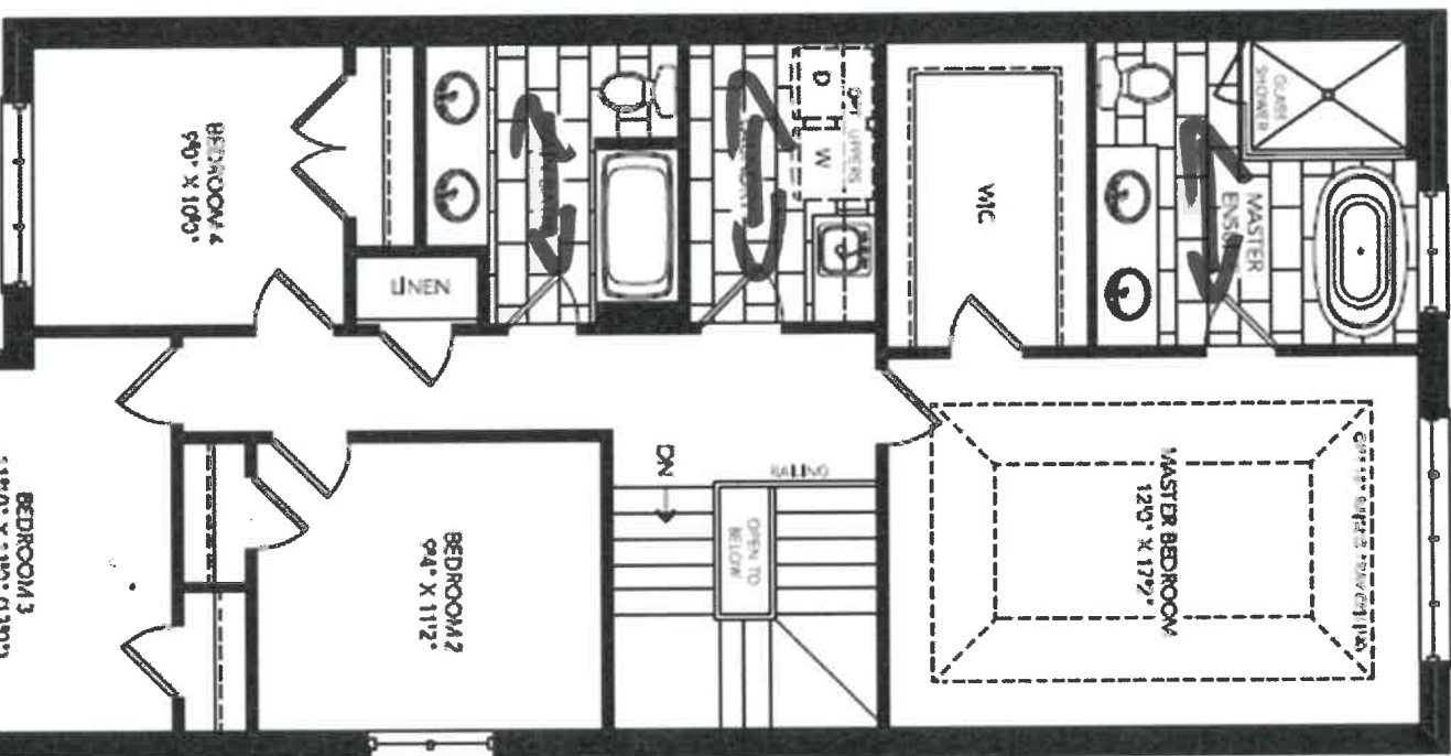
OPT. SECOND FLOOR PLAN 4 BEDROOM ELEV. B
