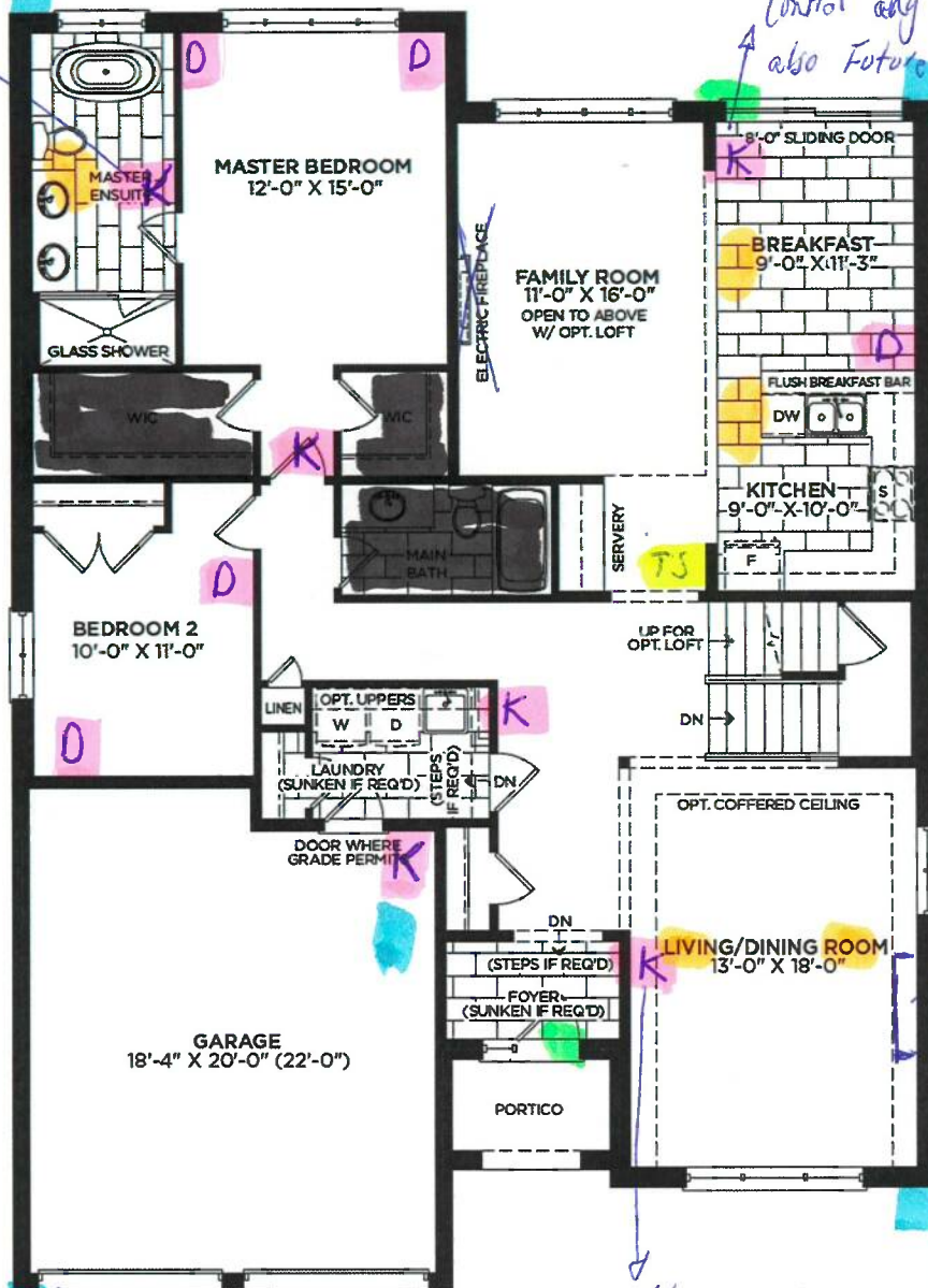
MAIN FLOOR ELEVATION A
