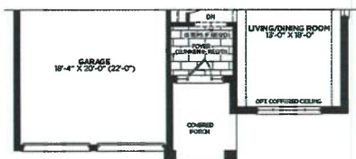
MAIN FLOOR ELEVATION C
