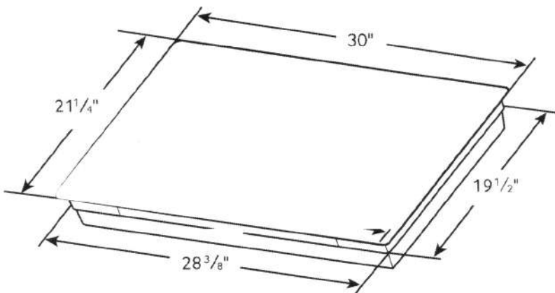
Cooktop Dimensions
